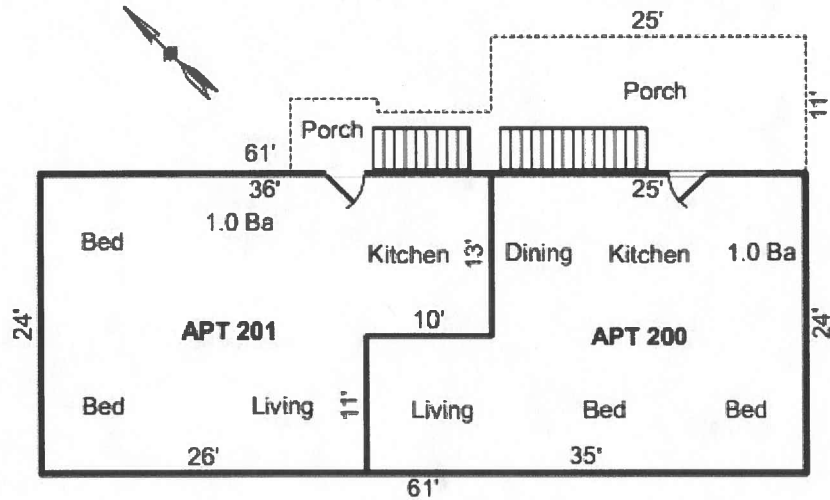
Building Diagram
